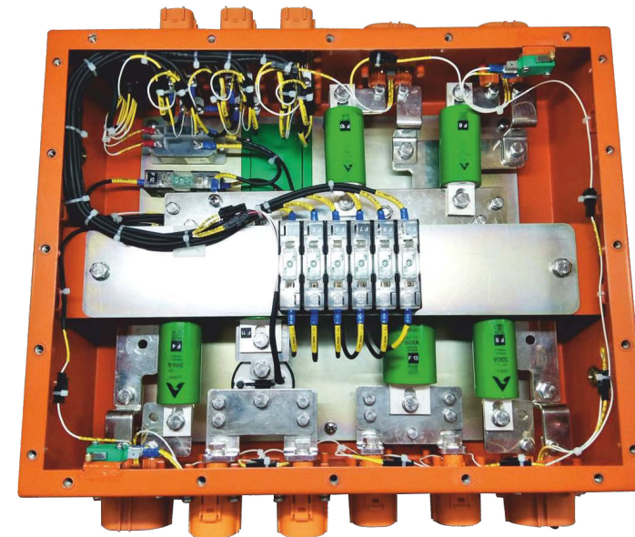
Electric Vehicle PDU
