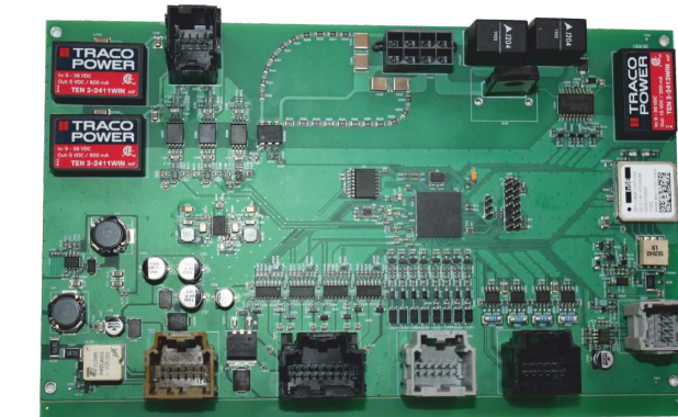
EV Battery Management System
